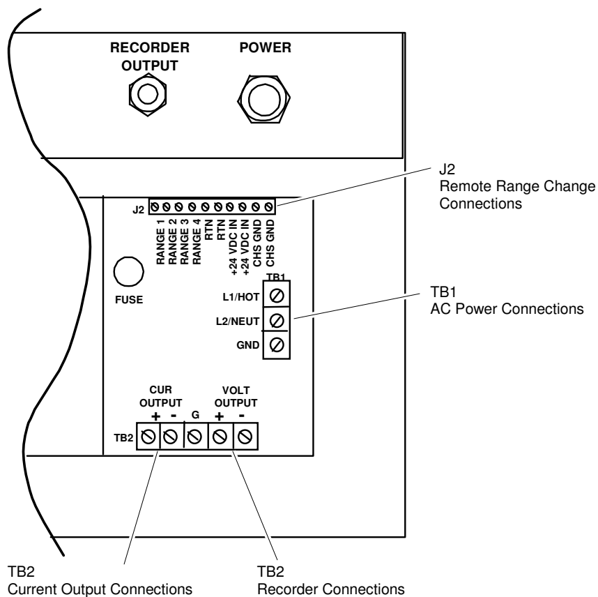
Figure 2-5. Rear Panel Wiring Connections
